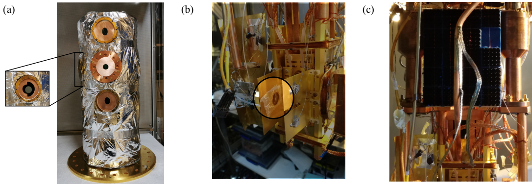
FIGURE IV.1 In (a), the Helium screen is shown where the copper irises are installed. In (b), the hole in the shield electrode covered with the thin mesh is show. In (c),we show a photograph of the MW absorber installation.
