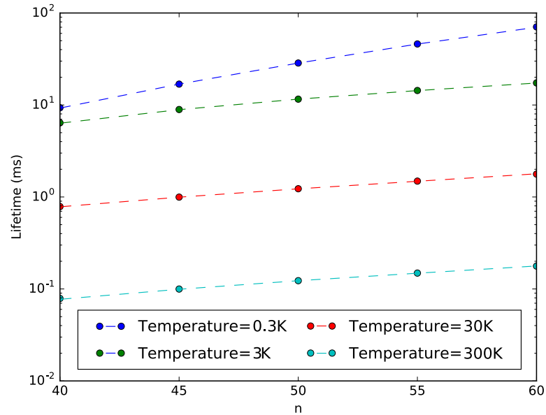
FIGURE II.7 Lifetime in free space as a function of the principal quantum number for a few temperatures. The dashed lines are guides to the eye. At low temperatures, spontaneous emission is dominant and the scaling is n^5 . At ‘high temperature’ ( T \geq 3 K), stimulated emission is dominant and the decay rate is suppressed by a factor of n_{th} \sim n^3 . The scaling becomes n^2 producing the parallel lines in the plot.
