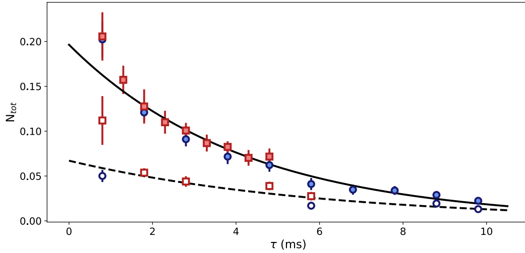
FIGURE V.15 Total population of |50c\rangle before the MW_P probe pulse for trapped (blue circles) and untrapped (red rectangles) atoms. The line is an exponential fit. Full symbols correspond to an average atom number \bar{N} . Open symbols correspond to measurements with about \bar{N}/2 atoms.
